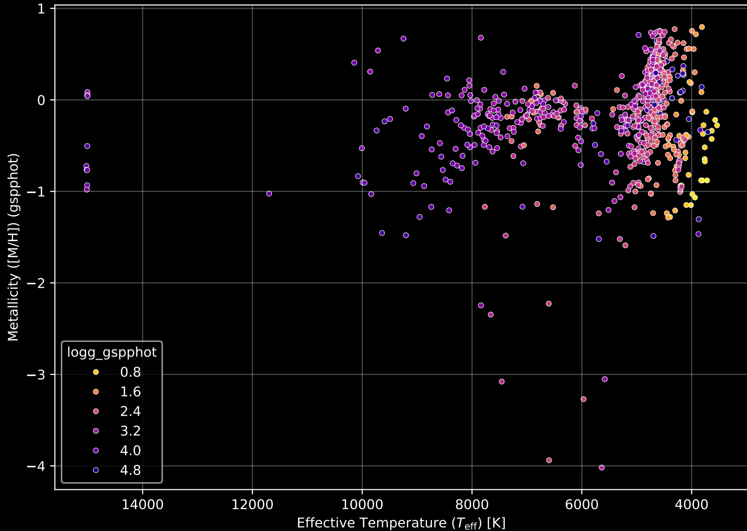
APOGEE DR17 Field: [270+00] Stellar Population Parameters (n= 741)
