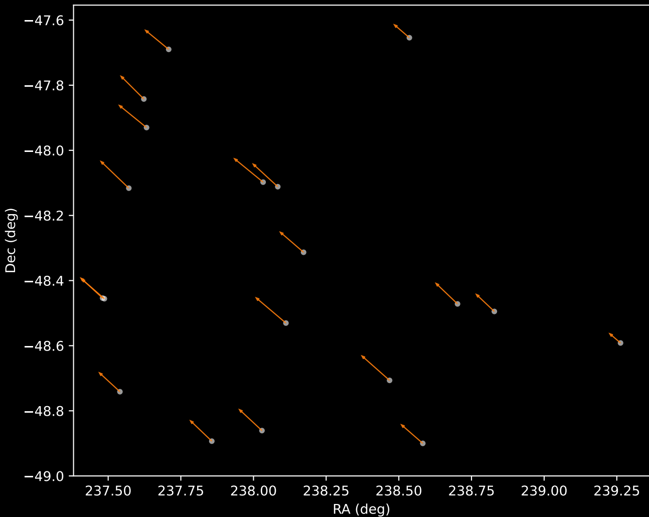
APOGEE DR17 Cluster 22 Proper Motion Vectors (n=19)
