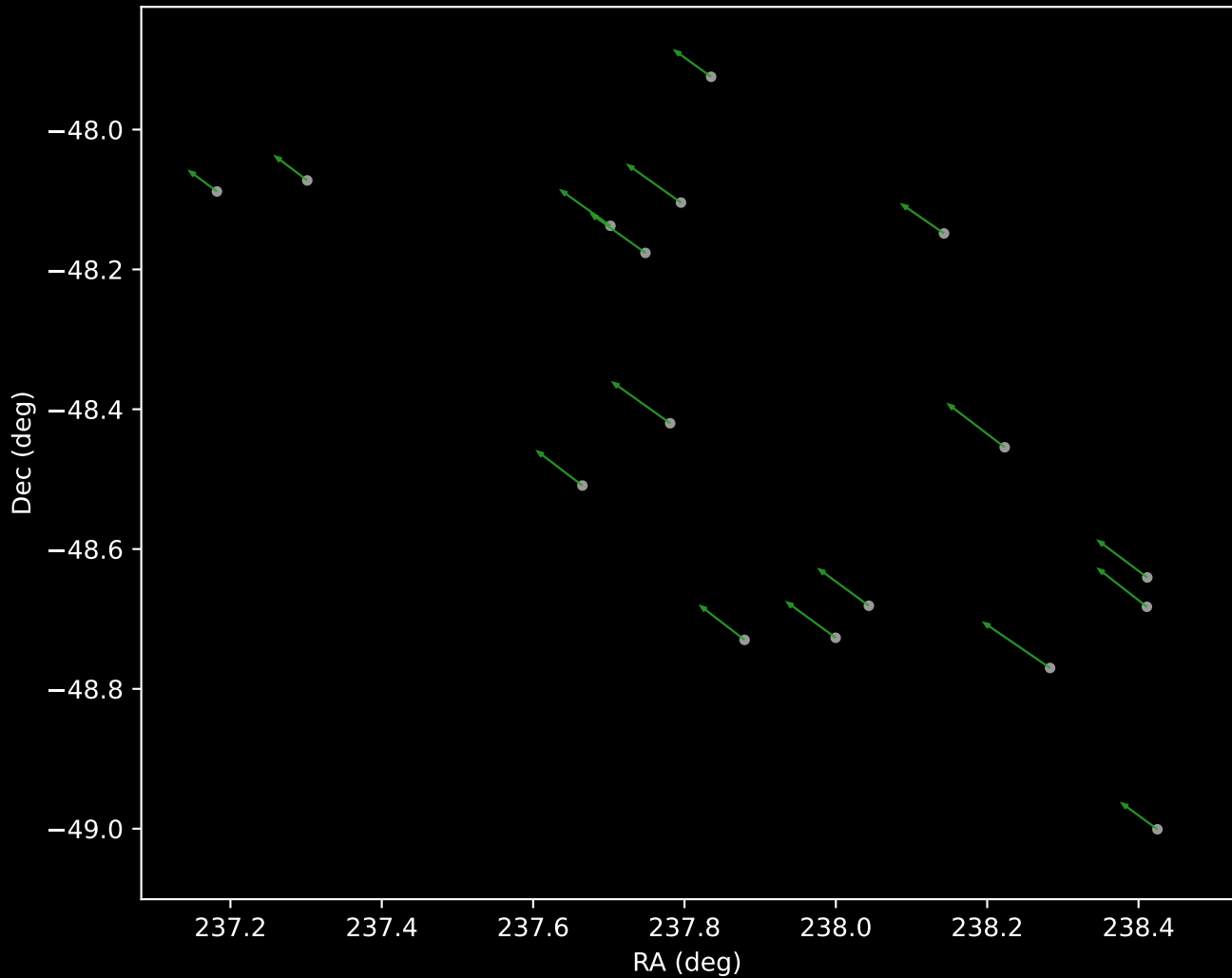
APOGEE DR17 Cluster 24 Proper Motion Vectors (n=17)
