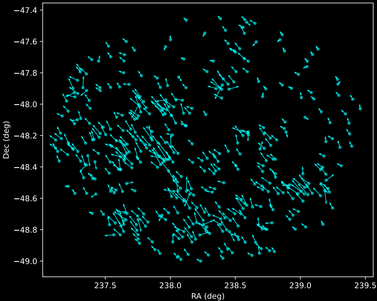
APOGEE DR17 Noise Stream Proper Motion Vectors (n=409)
