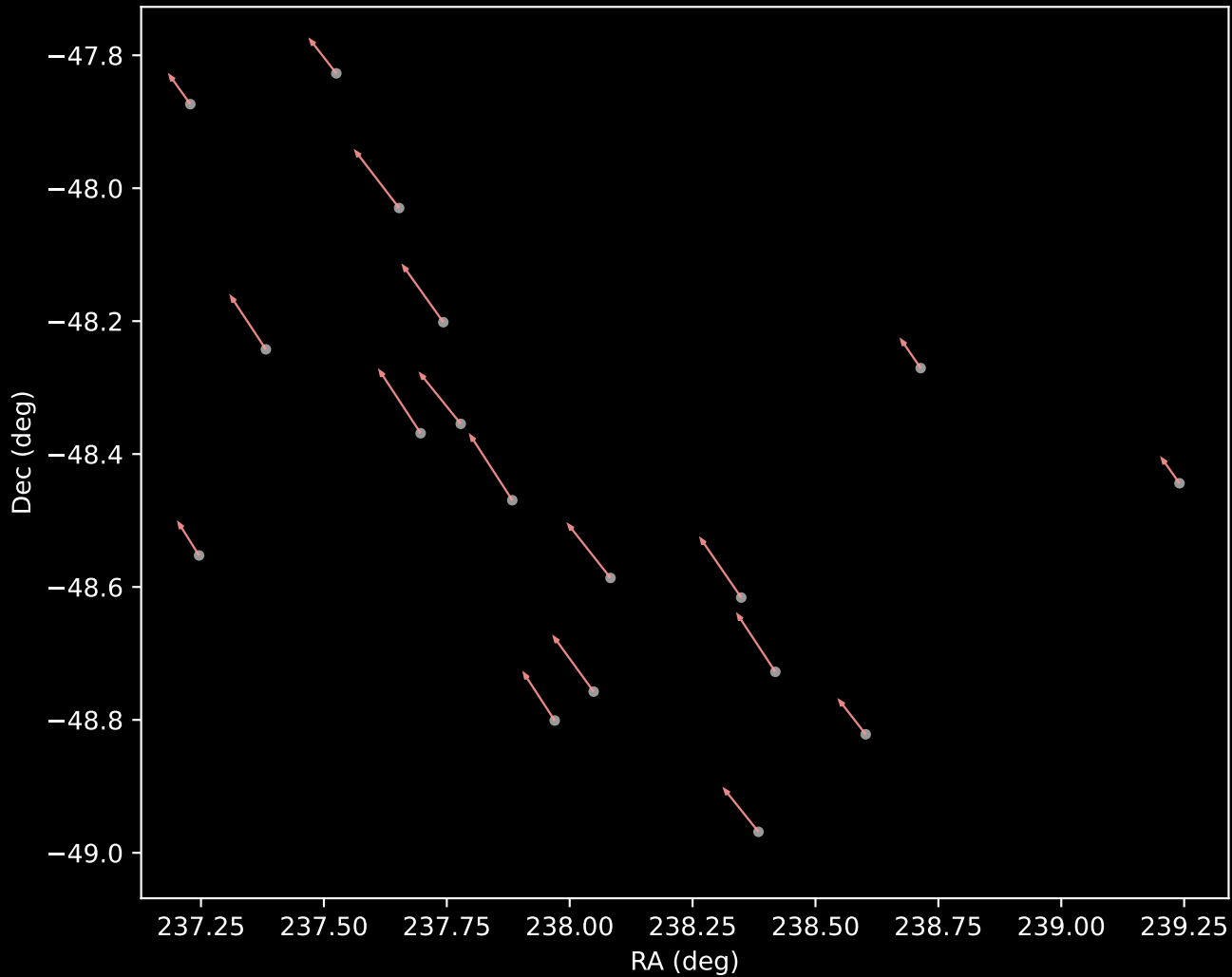
APOGEE DR17 Cluster 27 Proper Motion Vectors (n=18)
