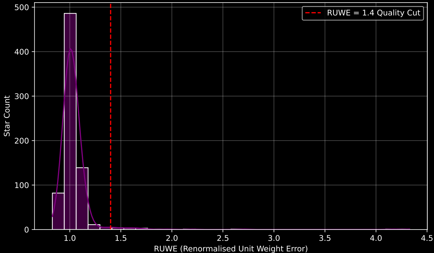
GAPOGEE DR17 Field [270+00] RUWE Distribution (n= 739)
