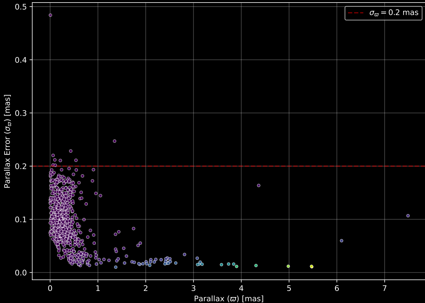
APOGEE DR17 Field: [270+00] Parallax Quality (n= 741)
