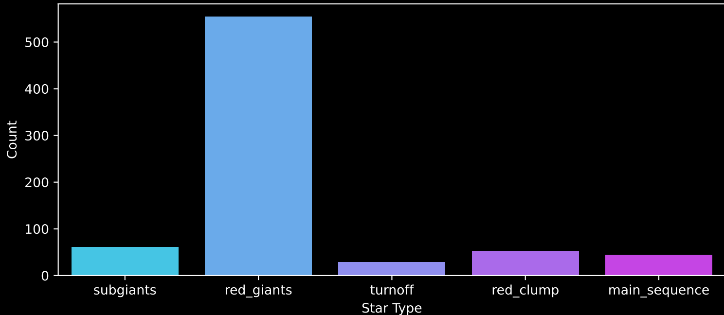
APOGEE DR17 Field: [270+00] Count plot of Star Type
