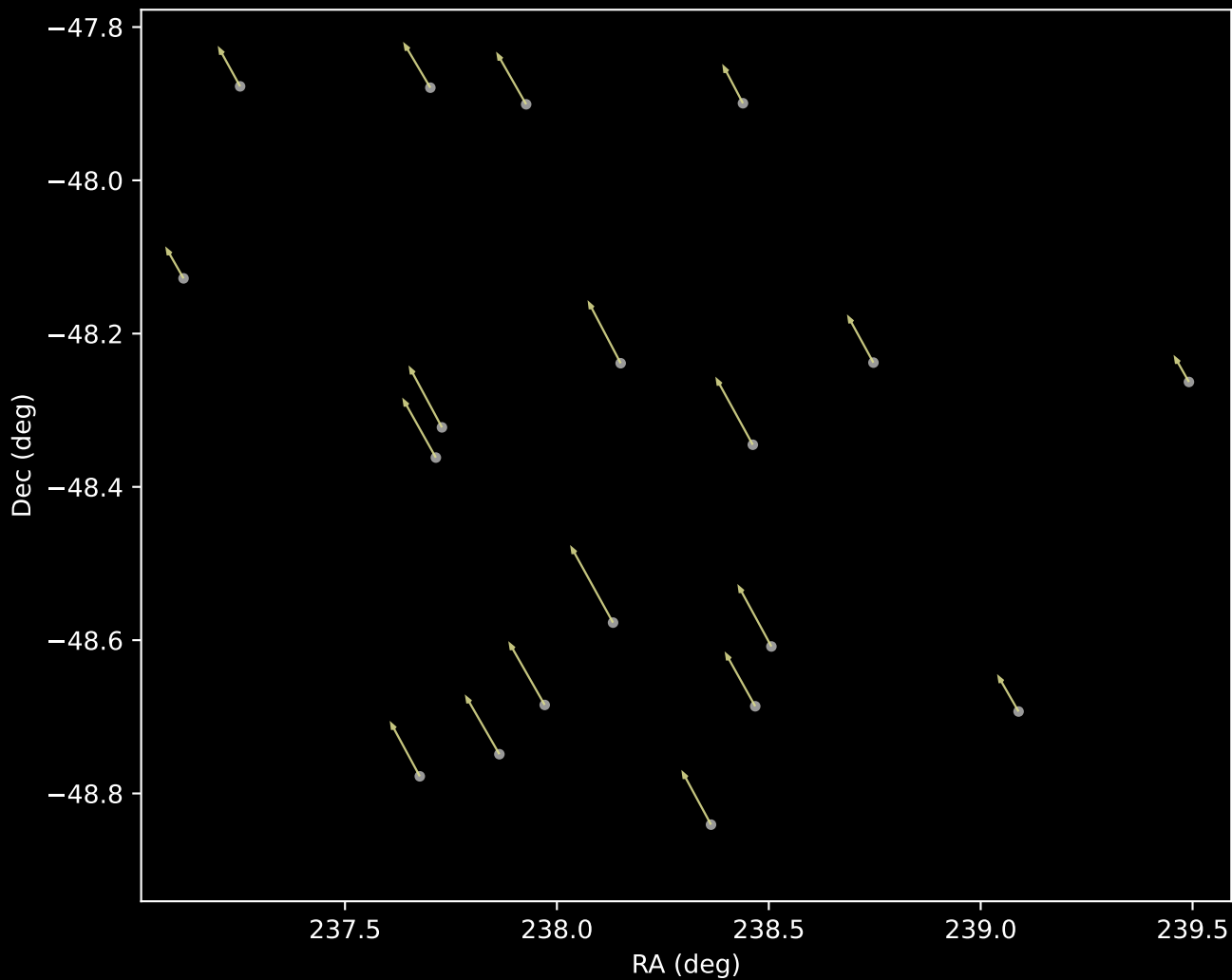
APOGEE DR17 Cluster 17 Proper Motion Vectors (n=19)
