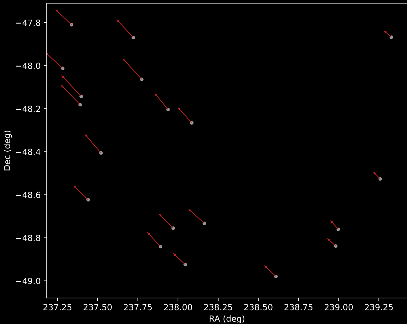
APOGEE DR17 Cluster 26 Proper Motion Vectors (n=19)
