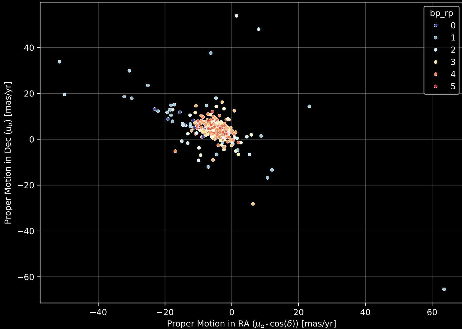
APOGEE DR17 Field: [270+00] Proper Motion Diagram (n= 741)
