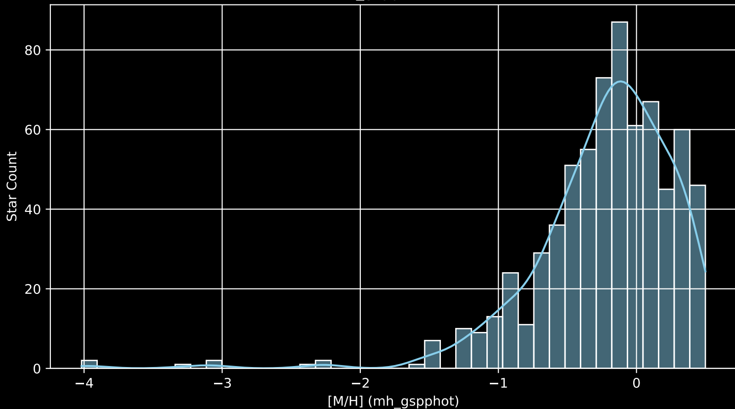
APOGEE DR17 Field: [270+00 [M/H] (mh_gspphot) (n= 693)
