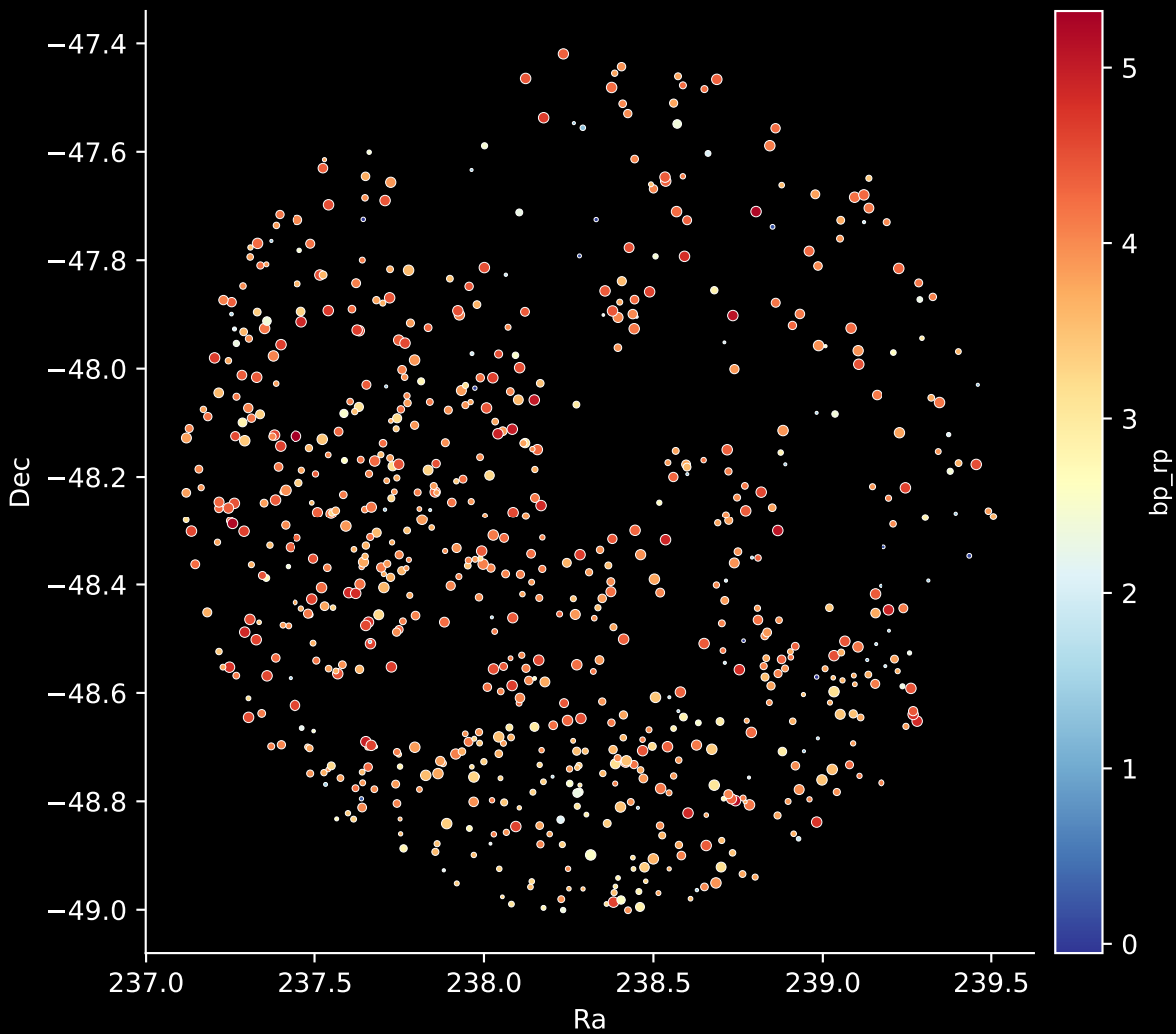
APOGEE DR17 Field: [270+00] Stars: 741
